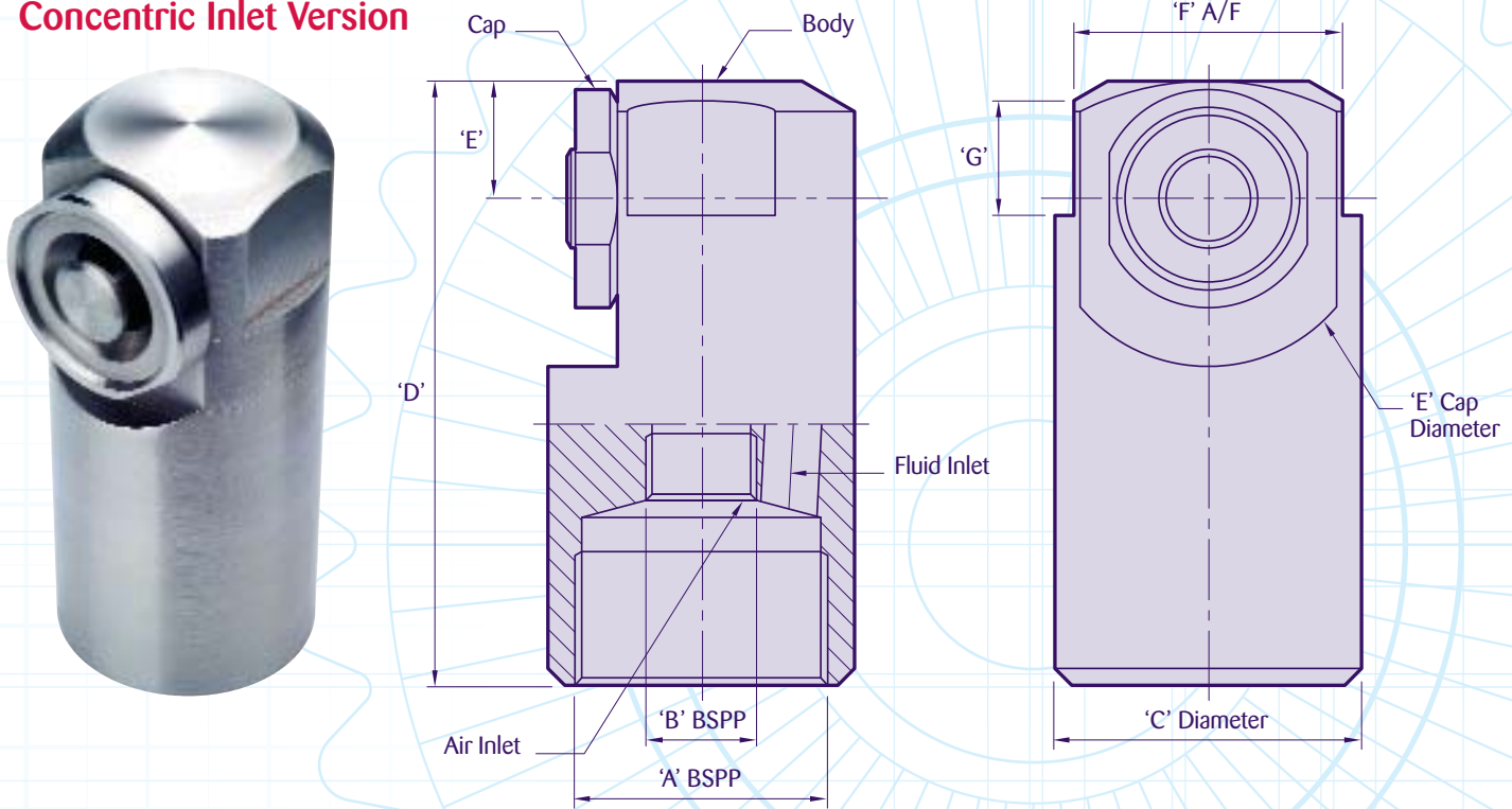
Concentric Inlet Nozzle Assembly Dimensions (inches/mm)
