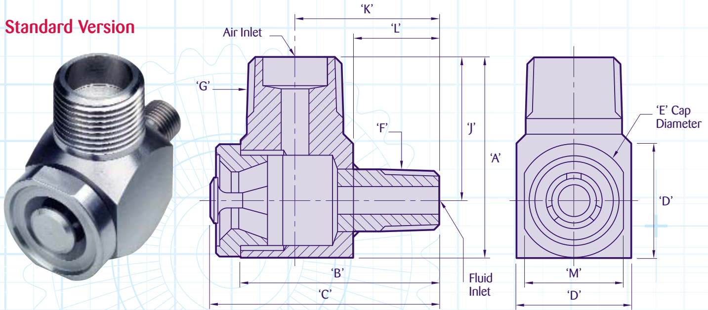
Right Angle Nozzle Assembly Dimensions (inches/mm)
